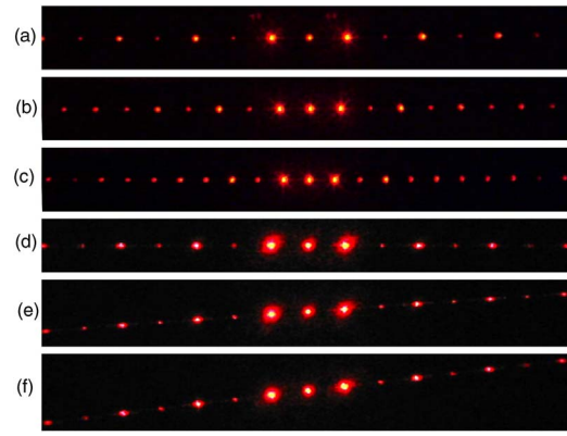
FIG. 3. (Color online) Photographs of diffraction patterns generated at different pressures P by the diffraction gratings engraved in the membranes of the stretcher [(a)–(c)] and of the rotator [(d)–(f)]. The pressures are (a) 0, (b) 0.75\ \text{psi} , (c) 1.5\ \text{psi} , (d) 0, (e) 0.75\ \text{psi} , and (f) 1.5\ \text{psi} .
