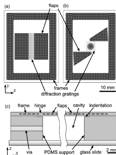
FIG. 1. Composite membrane devices, the stretcher and rotator. [(a) and (b)] Schematic drawings of the composite membranes in the stretcher and rotator, respectively. Dark areas correspond to epoxy parts inside the membranes. (c) Schematic drawing showing a cross section of a device.
