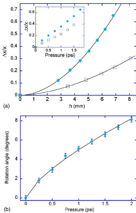
FIG. 4. (Color online) (a) Relative extension of the central strips, \Delta x/x_0 , as a function of elevation of the center of the membrane, h , for the stretcher (circles) and for the plain membrane device (squares). The continuous lines are power law fits, \Delta x/x_0 \propto h^{1.9} and \Delta x/x_0 \propto h^{1.7} , for the composite and plane membrane devices, respectively, shown to guide the eyes. Error bars are smaller than symbols and are not shown. Inset: \Delta x/x_0 as a function of pressure P for the stretcher (circles) and for the plain membrane device (squares). Error bars are smaller than symbols and are not shown. (b) Angle of the in-plane rotation \varphi of the central circle of the composite membrane in the rotator as a function of pressure P applied to the device. The continuous line is a power law fit, \varphi \propto P^{0.72} , shown to guide the eyes.
