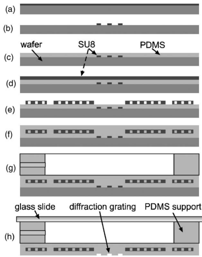
FIG. 2. Fabrication of a composite membrane device is shown step by step from top to bottom.
